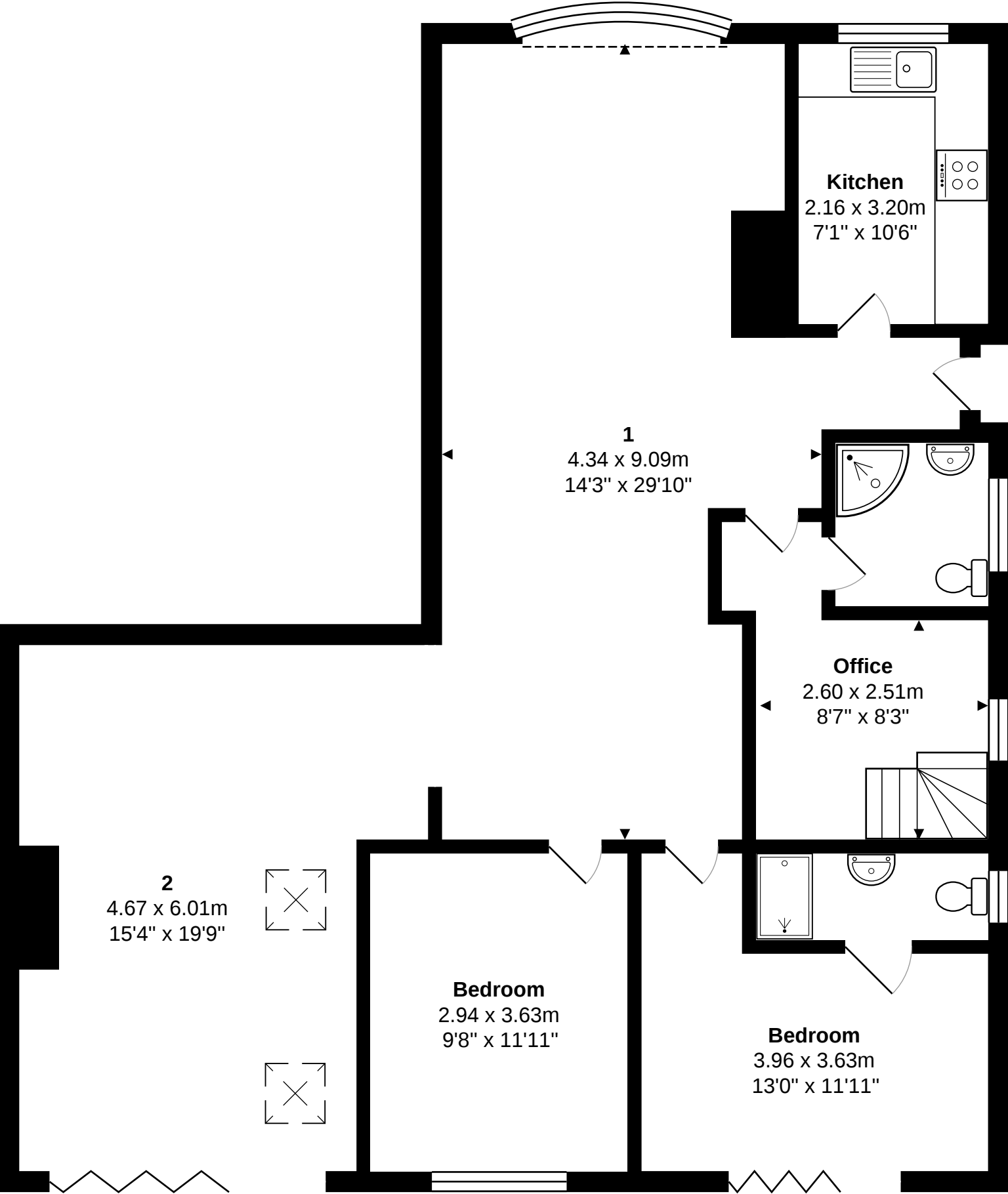
Ground Floor
